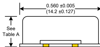
Package Height Options (Max)
